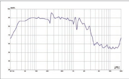
Frequency Response Curve
