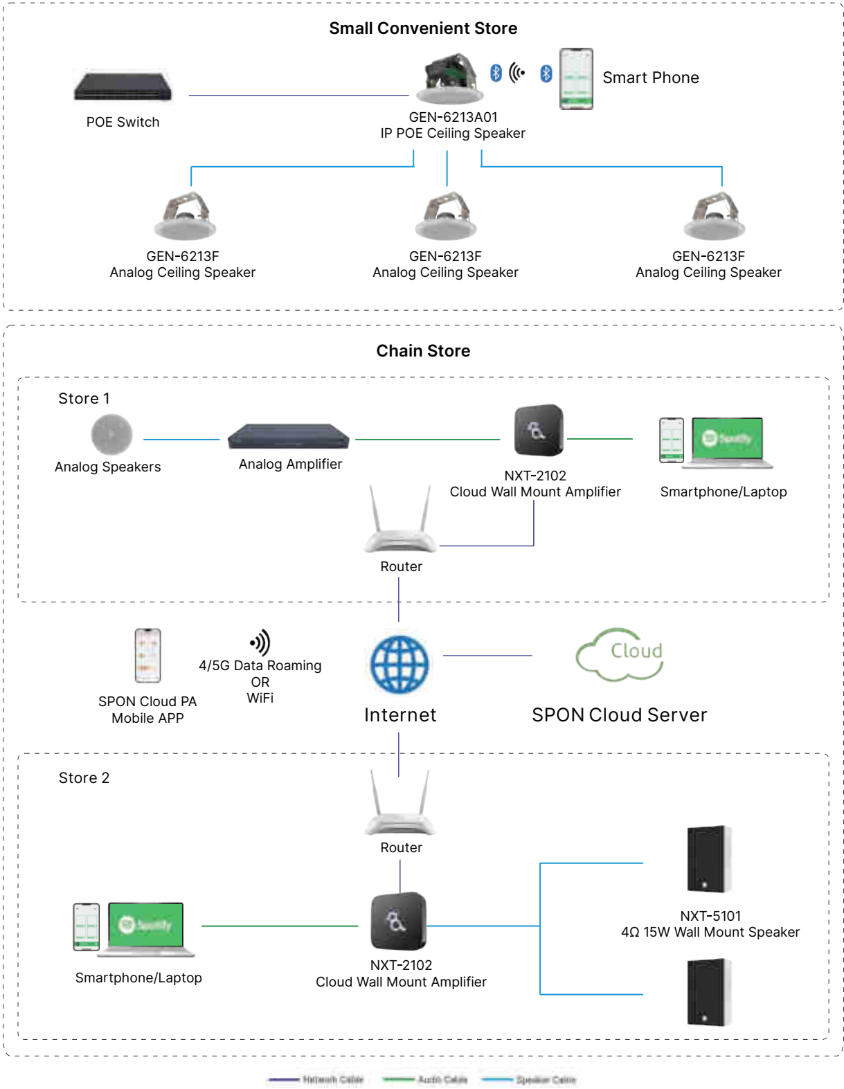
Topology Diagram
