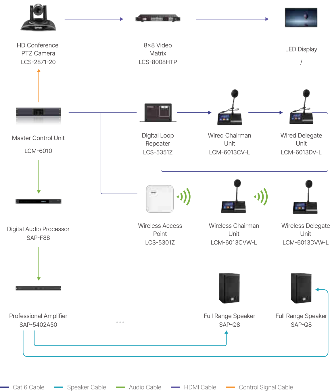
Topology Diagram
