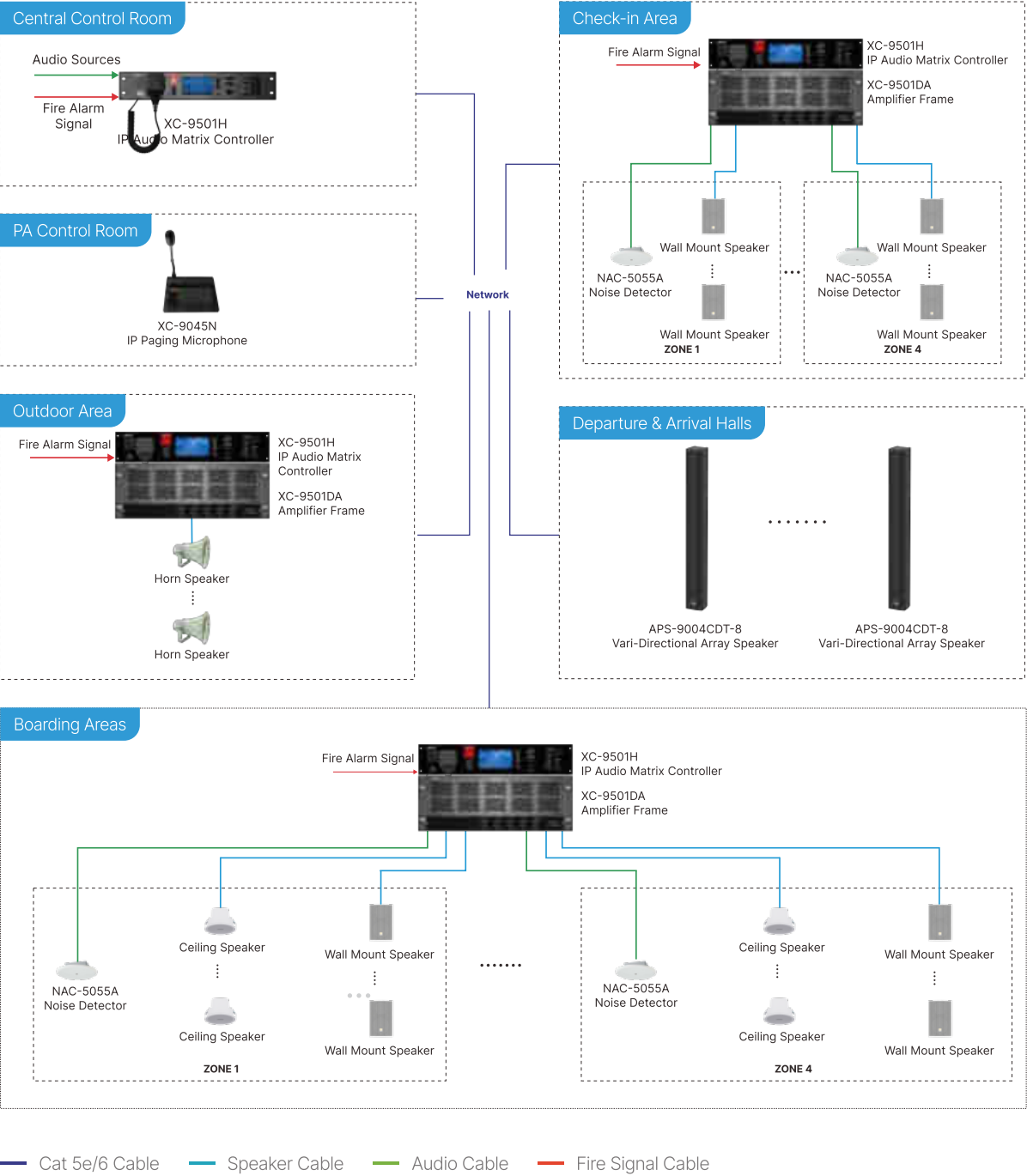
Topology Diagram
