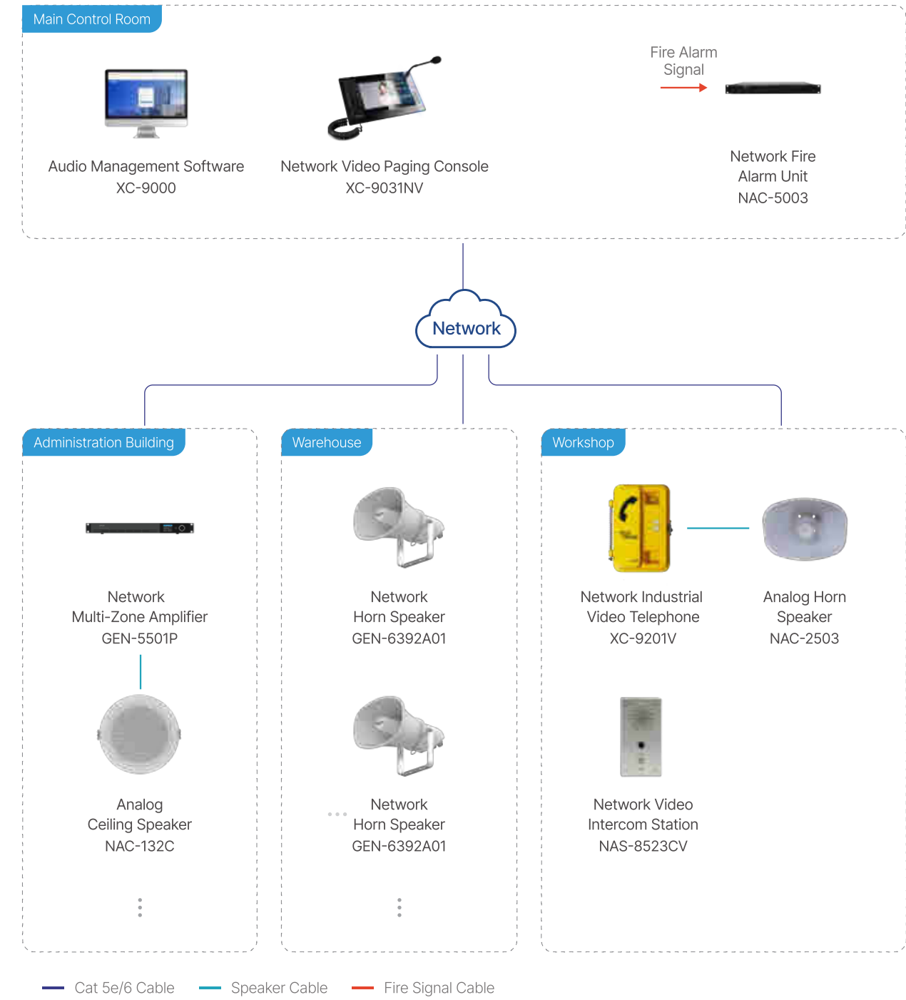
Topology Diagram
